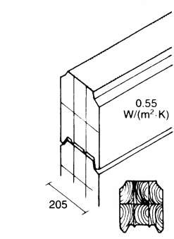
⑰ Profiled laminated timber log construction 0.55 W/(m 2 ·K)
